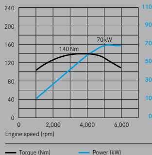
A 160 BlueEFFICIENCY
