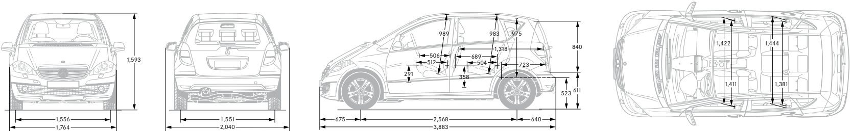
All measurements in millimetres. Measurements shown are average values applicable to unladen standard models
